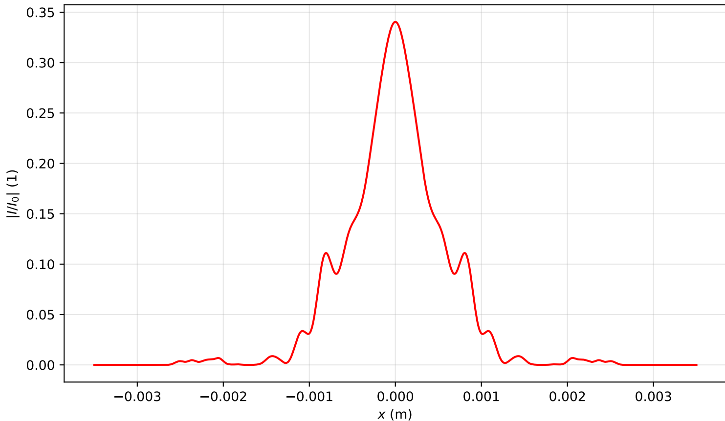
Intensity profile I(x, y = 0, z = 1.672)/I_0 , P_{in}=7.0P_{cr} , artificial time
